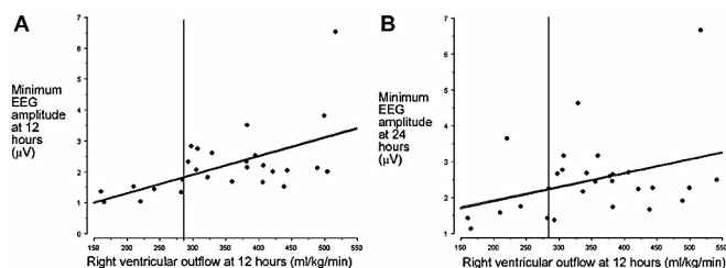
Figure 1. Relationship between RVO at 12 h and minimum EEG amplitude measurements at 12 h (A) ( n = 27 , r^2 = 0.31 ) and 24 h (B) ( n = 30 , r^2 = 0.15 ), with vertical line indicating cutoff for lowest quartile of outflow measurements (<282 mL/kg/min).
