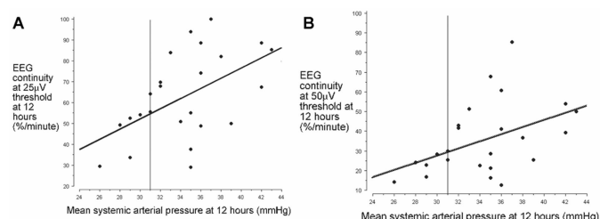
Figure 2. Relationship between mean systemic arterial blood pressure at 12 h and EEG continuity measurements at 12 h at the 25 \mu V (A) ( n = 27 , r^2 = 0.28 ) and 50 \mu V (B) ( n = 27 , r^2 = 0.20 ) thresholds, with vertical line indicating cutoff for lowest quartile of pressure measurements (<31 mm Hg).
